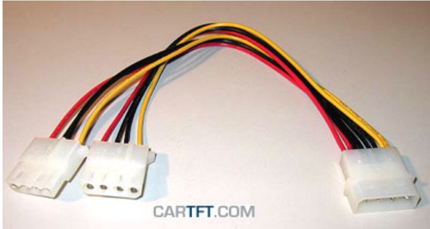
Y-Power Divider 5.25" to 2x 5.25"
